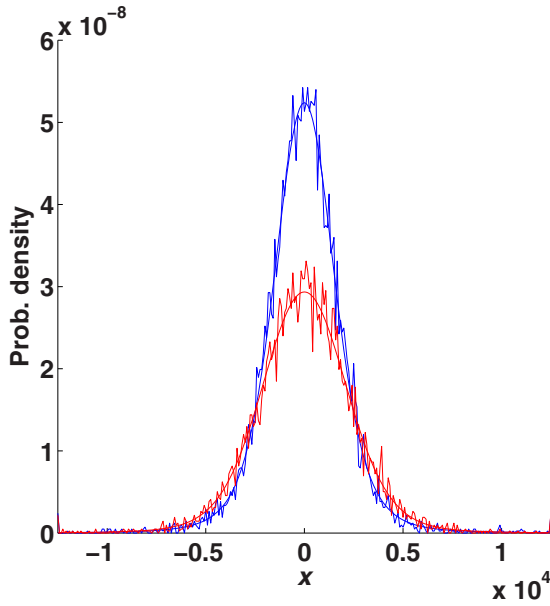
FIG. 3. Cross section of m^0(t, \mathbf{x}) for varying \kappa . For \kappa = 0 , the smooth blue (top) curve shows the analytic solution for m^0 ; the jagged blue (top) curve shows the simulation constructed m^0 . For \kappa = 10 , the smooth red (bottom) curve shows the analytic solution for m^0 ; the jagged red (bottom) curve shows the simulation constructed m^0 . Full details in main text.
