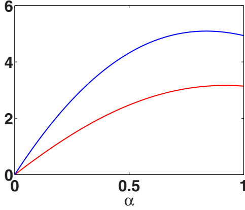
FIG. 1. Plot of the function \Upsilon_d(\alpha) for 0 < \alpha < 1 with d = 2 (red, bottom) and d = 3 (blue, top).
