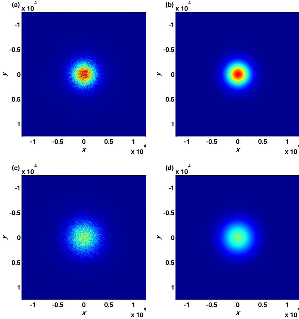
FIG. 2. Comparison of simulations of Algorithm I, see Appendix A, and analytic solution to m^0(t, \mathbf{x}) given by Eq. (39). Top row: case where \kappa = 0 , (a) simulation, (b) analytic solution. Bottom row: case where \kappa = 10 , (c) simulation, (d) analytic solution. Full details in main text.
