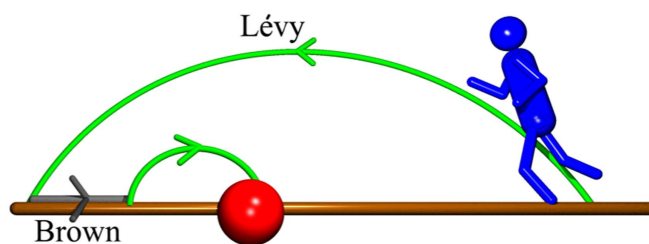
Figure 1. Sketch of intermittent search in one dimension: a searcher (blue) proceeds by a combination of Lévy jumps and Brownian steps until it finds the target (red). Physically, Lévy jumps decorrelate the motion, leading the searcher to sites not previously visited. Brownian motion, instead, provides a thorough local search at the price of oversampling, see text.
